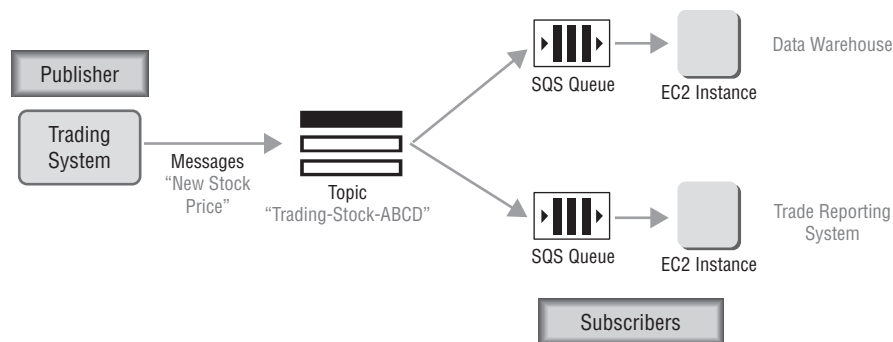
FIGURE 10.4 Fan-out scenario
