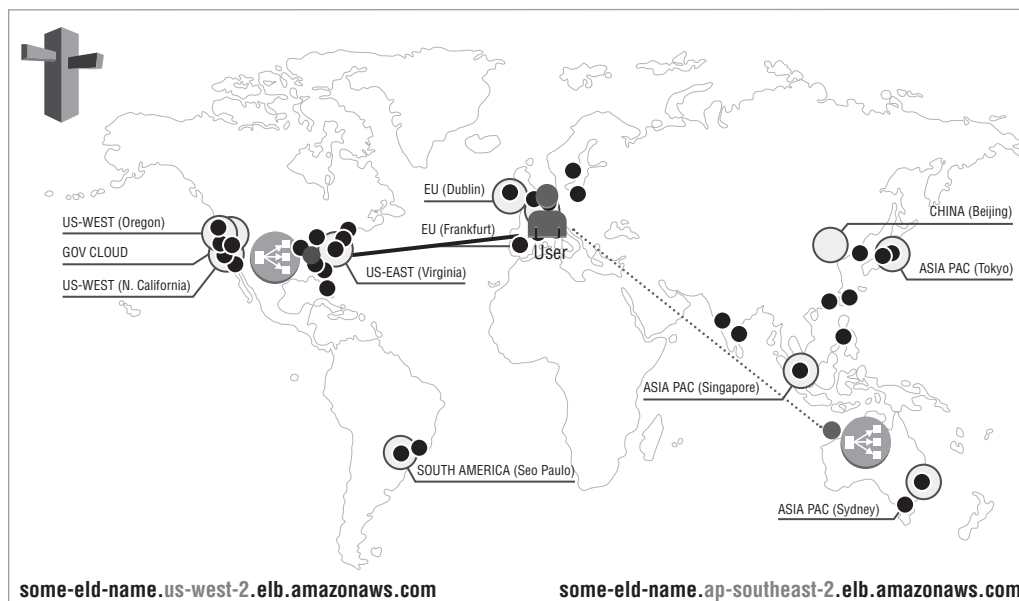
FIGURE 5.8 Weighted routing
