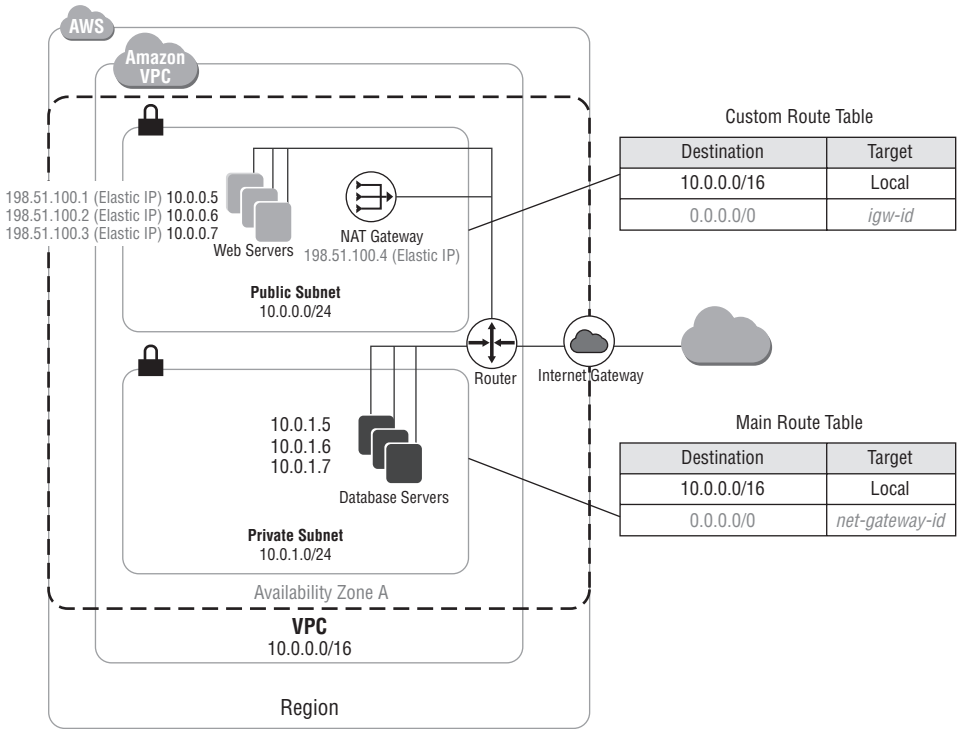
FIGURE 5.4 VPC diagram
